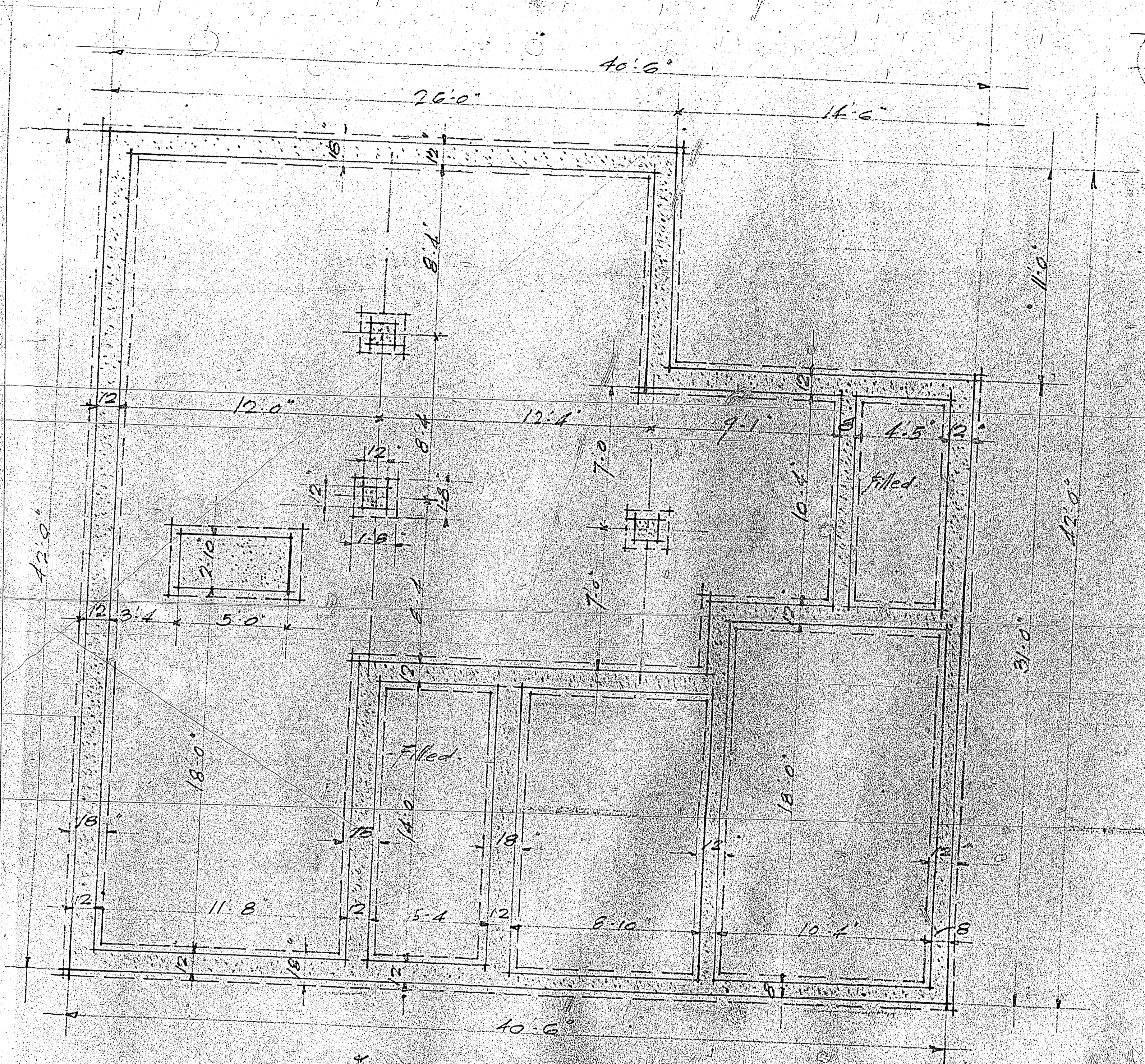
FOUNDATION PLAN Scale 1/4"
