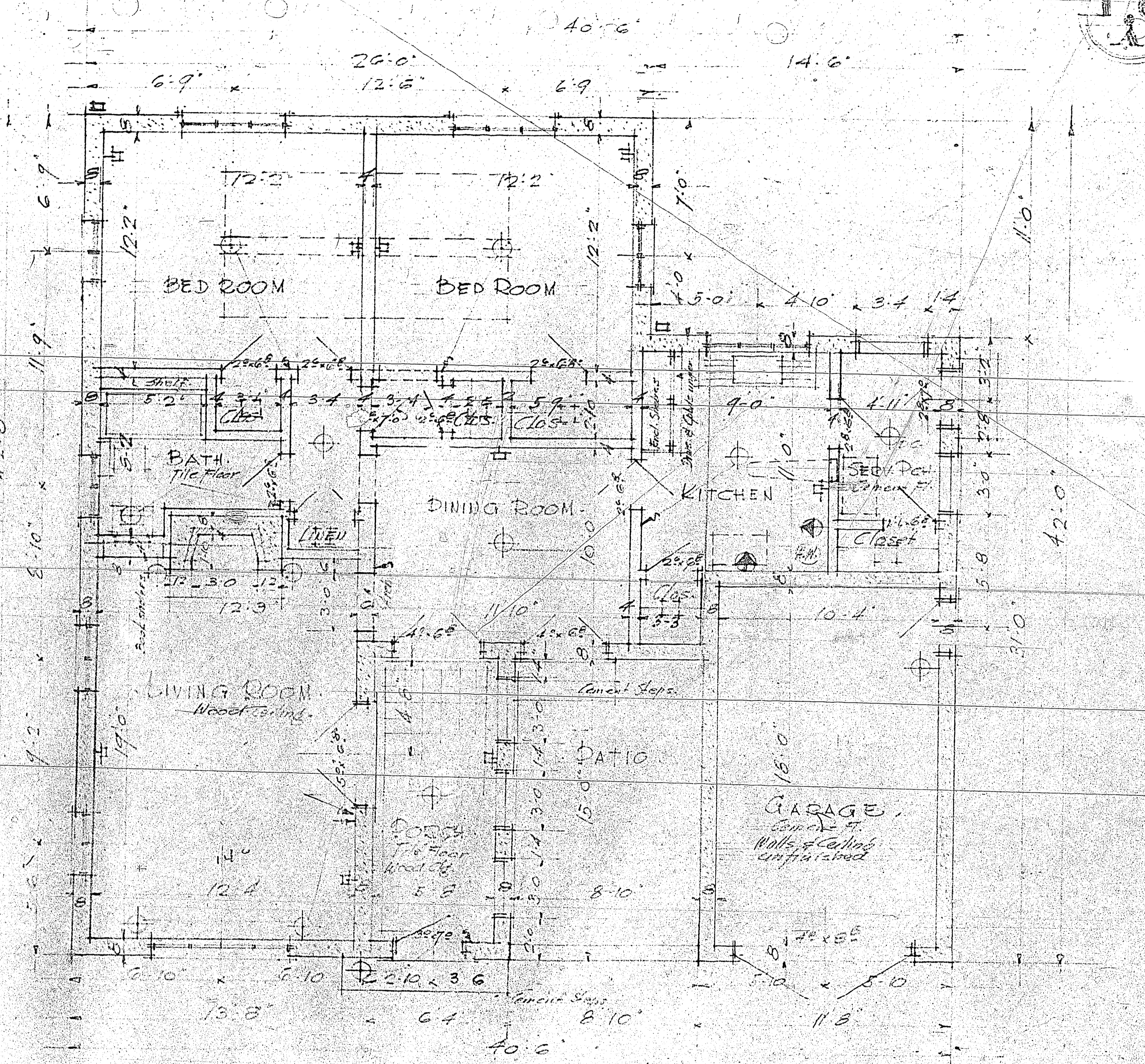
FIRST FLOOR PLAN Scale 1/4"
