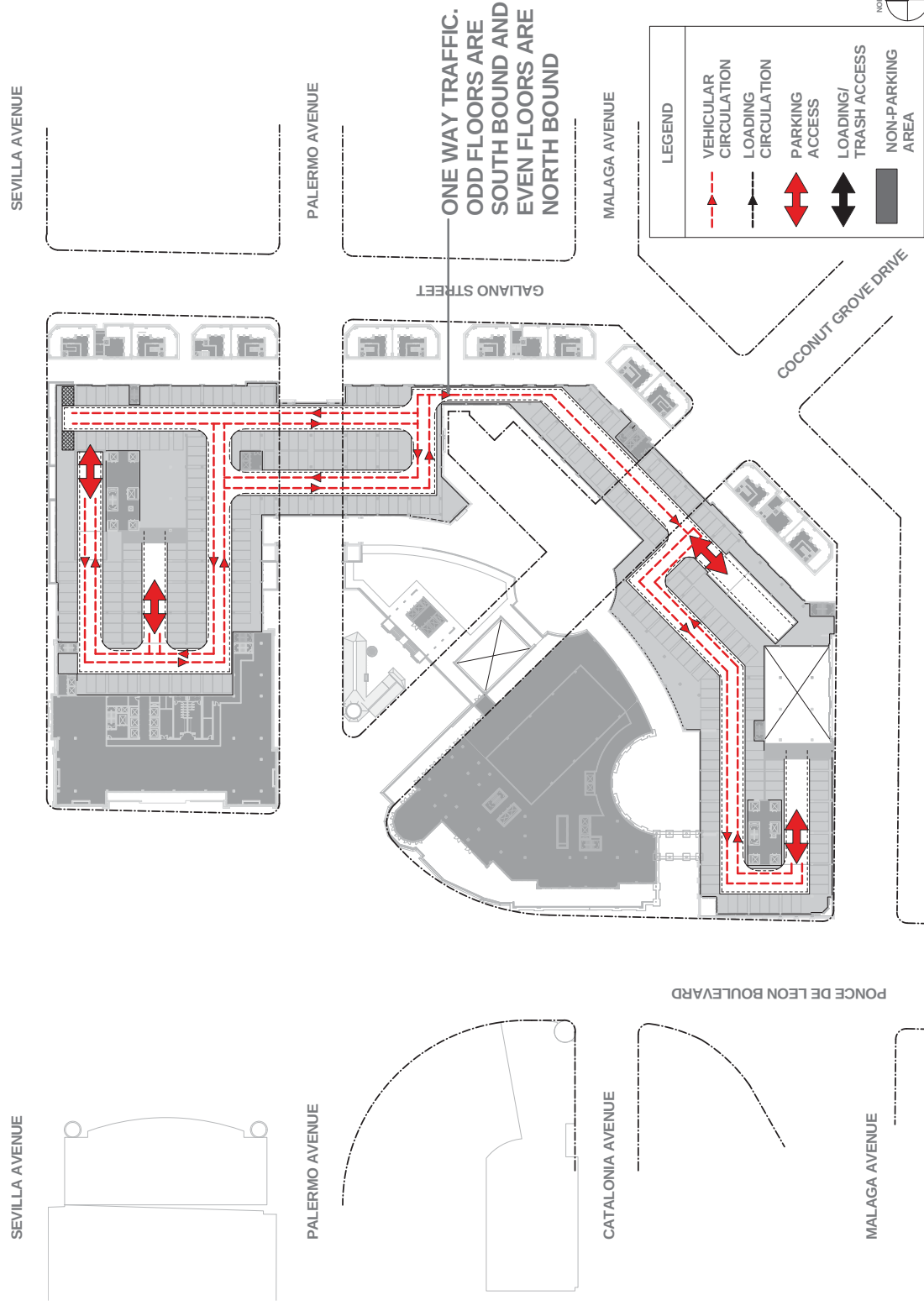
1 LEVEL 03 FLOOR PLAN 1/8" = 4'-0"
