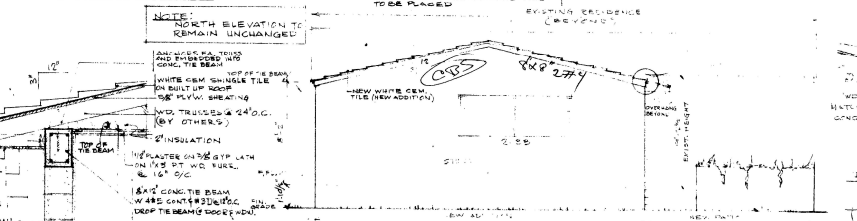
SOUTH ELEVATION 1/4"
