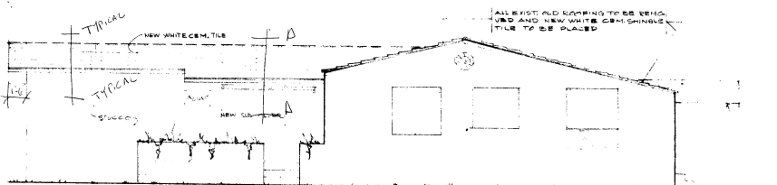
EAST ELEVATION 1/4"
