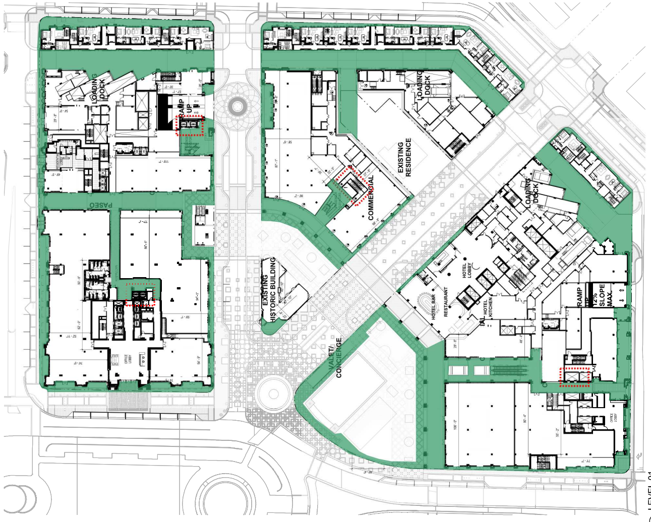
1 LEVEL 01 1/8" = 1' 0"
