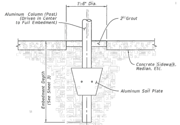
Driven Post Detail
