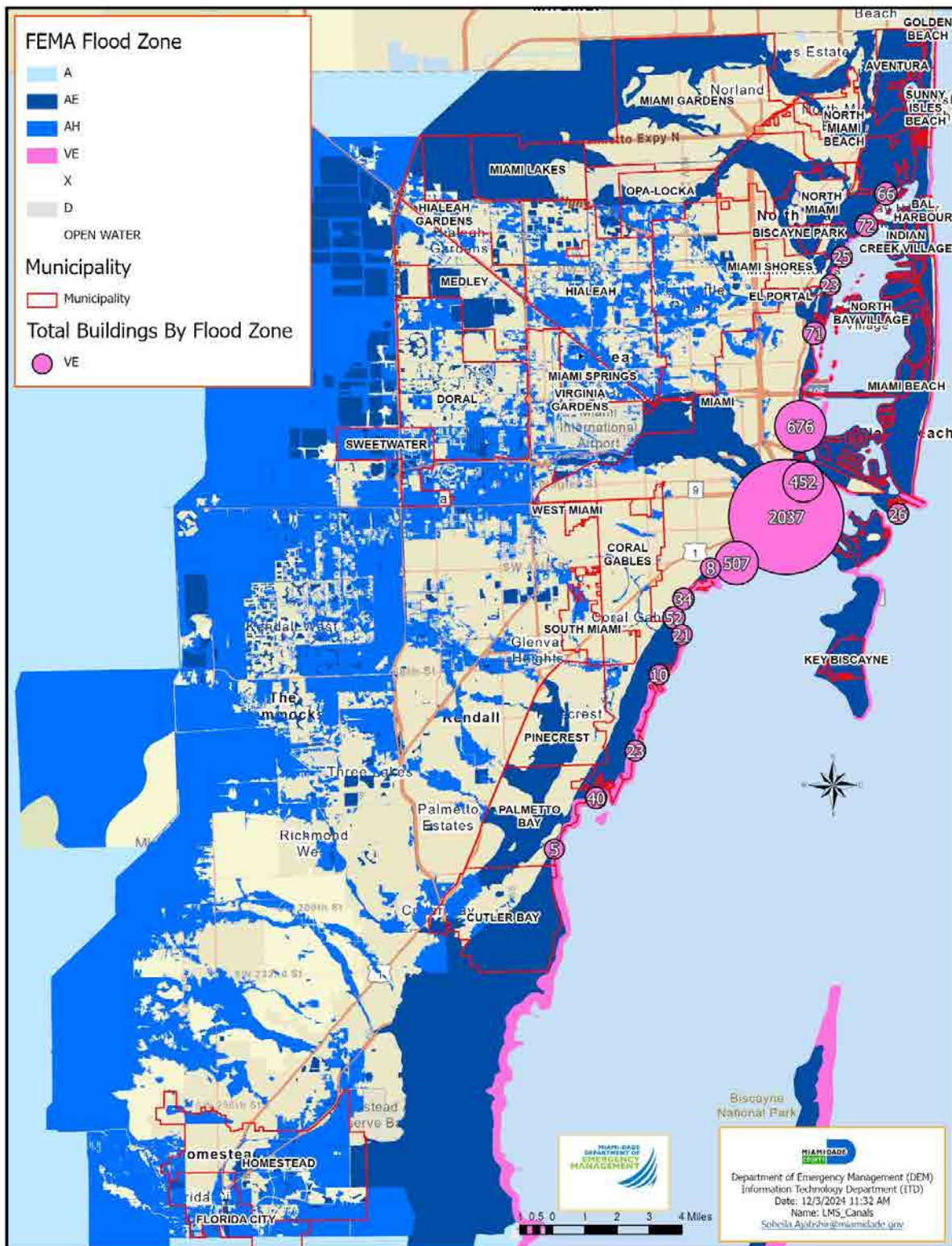
Figure 14. Buildings by FEMA Flood Zones – VE
