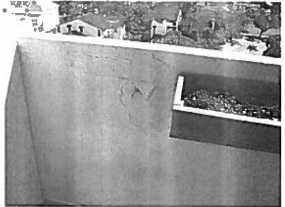
Figure 10- Spalled concrete railing-Unit 1205
