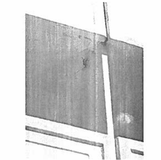
Figure 6-Spalls south balcony
