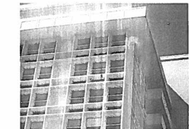
Figure 8-Spalls at Precast Beam at roof
