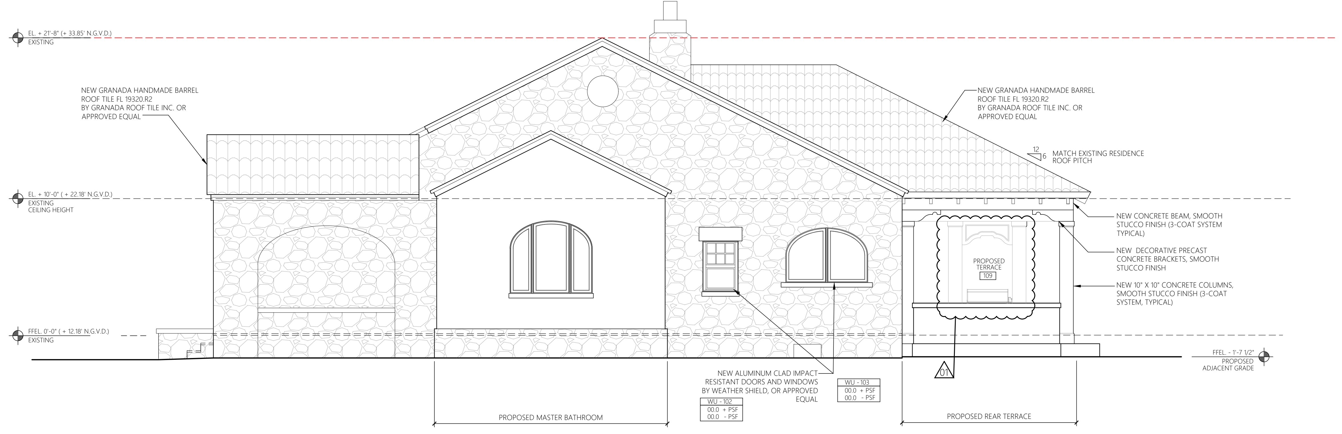
PROPOSED SIDE ELEVATION SCALE: 1/4" = 1'-0"
