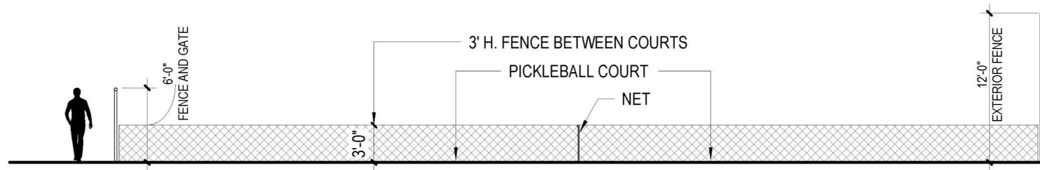
FENCE AND COURT DIMENSIONS
