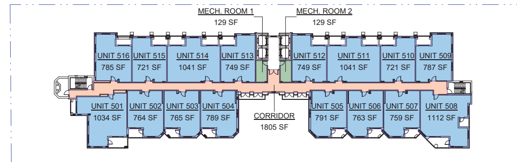
6 5th Level 1" = 30'-0"
