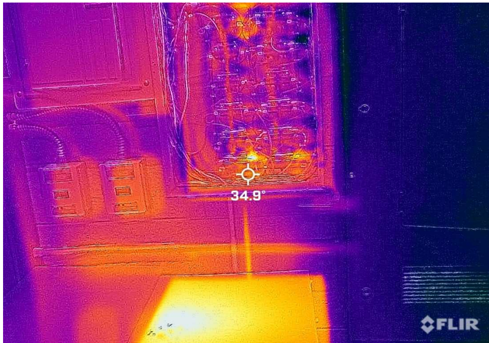
Item 9: Control Cabinet at 34.9 Degrees Celsius (delta 9.9C)
