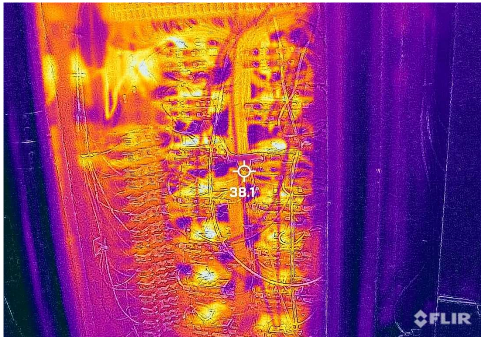
Item 65: Control Panel at 38.1 Degrees Celsius (delta 2.4C)
