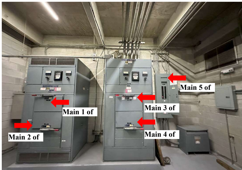
Switchgear Room Layout - Service Entrance – Mains 1 through 5
