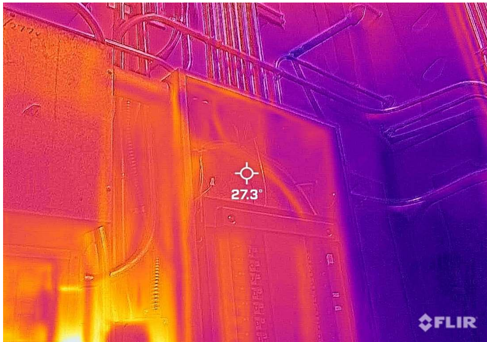
Item 59: Panel NH10 at 27.3 Degrees Celsius (delta 4.3C)
