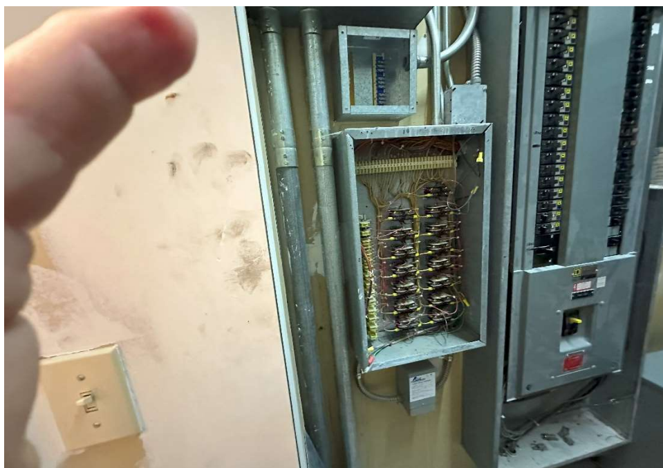
Relay Control Panel
