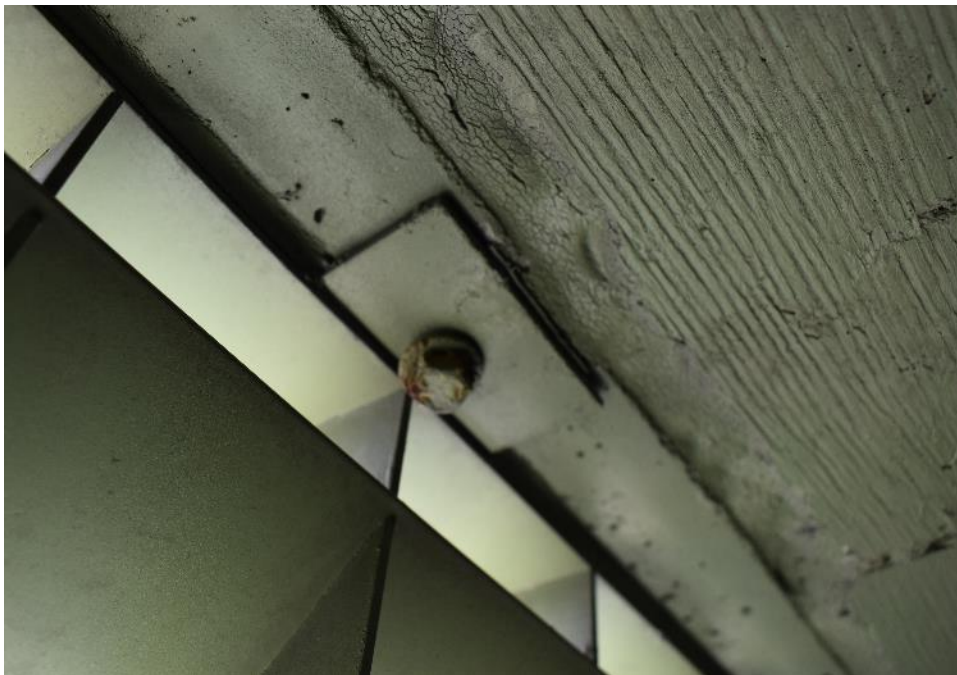
Typical louver connections at the garage level
