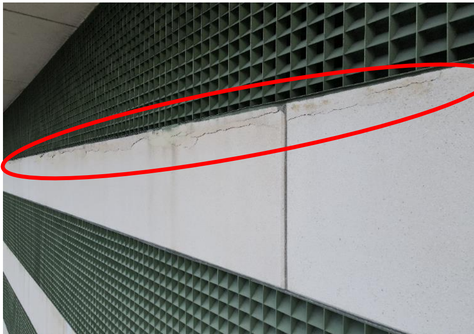
Cracking concrete at exterior walls of parking garage
