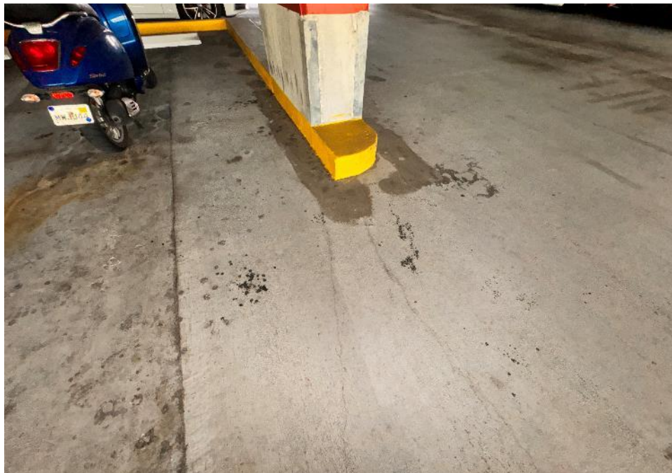
Typical linear cracks in the concrete decking at the garage levels
