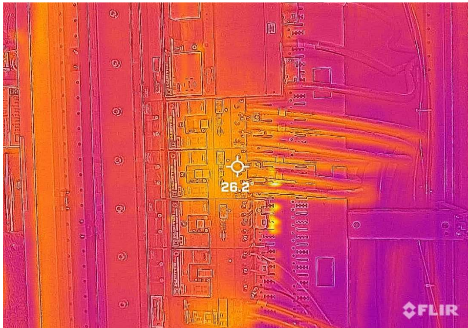
Item 35: Panel PH at 26.7 Degrees Celsius (delta 1.7C)
