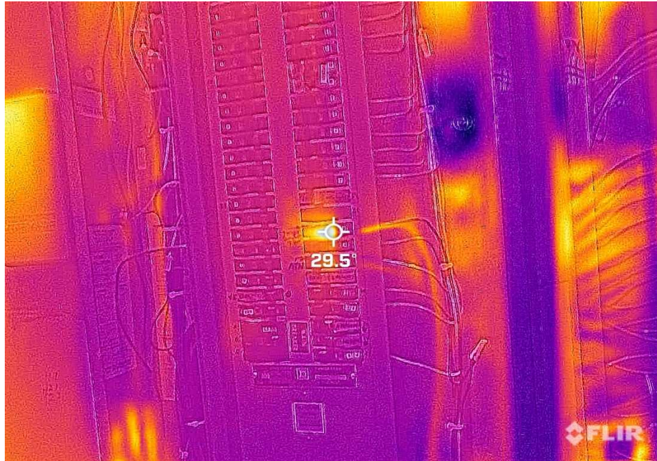
Item 39: Panel NL8 at 29.5 Degrees Celsius (delta 6.5C)
