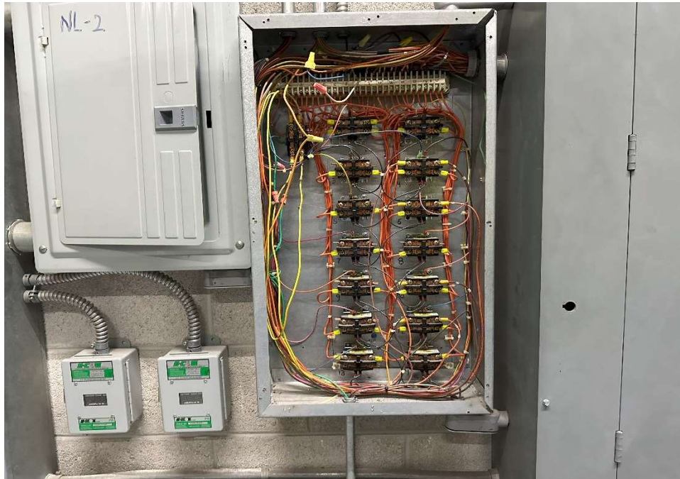
Control Cabinet Opened -
