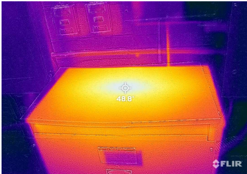
Item 12: T2 at 48.8 Degrees Celsius
