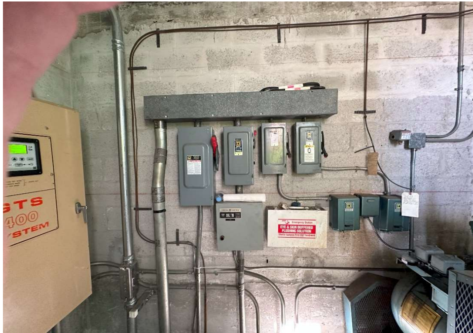
Elevator Machine Room Disconnects – Tied to Generator - Roof
