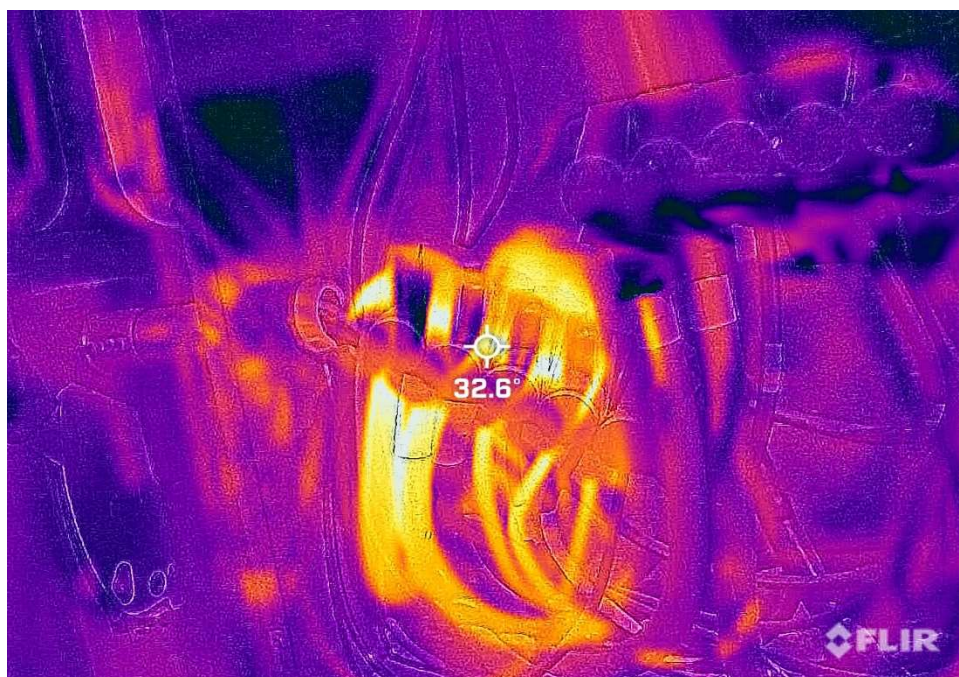
Item 44: J-Box at 32.6 Degrees Celsius (delta 9.6C)
