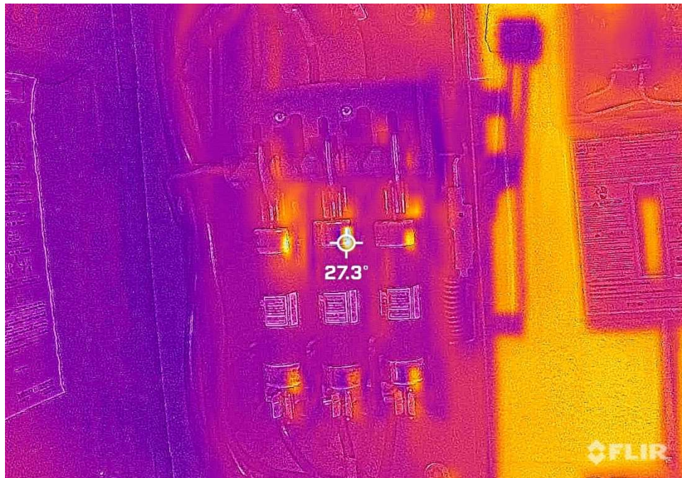
Item 24: Elev Disconnect 3 at 27.3 Degrees Celsius (delta 5.3C)
