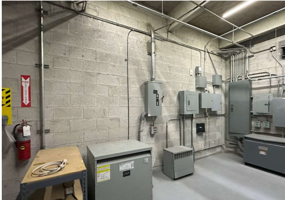
Switchgear Room Layout -
