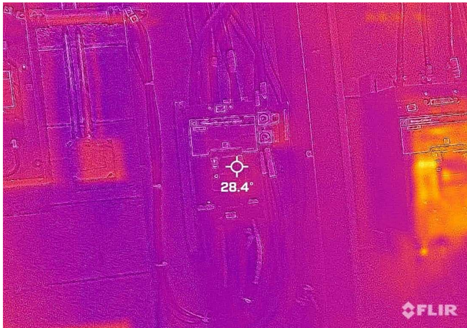
Item 19: ATS Disconnect at 28.4 Degrees Celsius (delta 3.4C)
