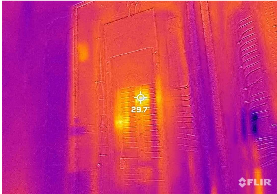
Item 48: Panel NL9A at 29.7 Degrees Celsius (delta 7.7C)
