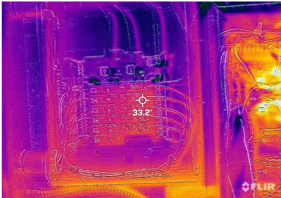
Item 10: Panel NL2 at 33.2 Degrees Celsius (delta 8.2C)
