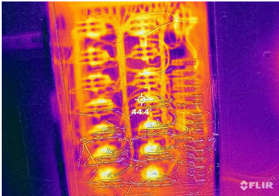
Item 78: Control Panel at 44.4 Degrees Celsius
