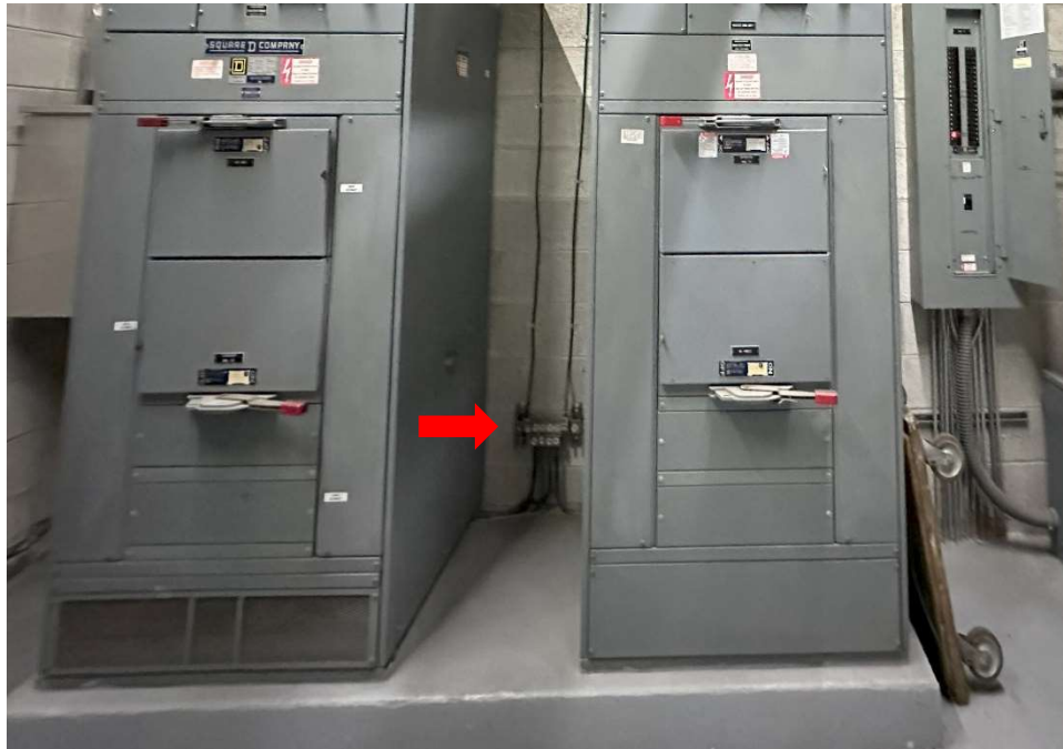
Electrical Service Ground Bus -
