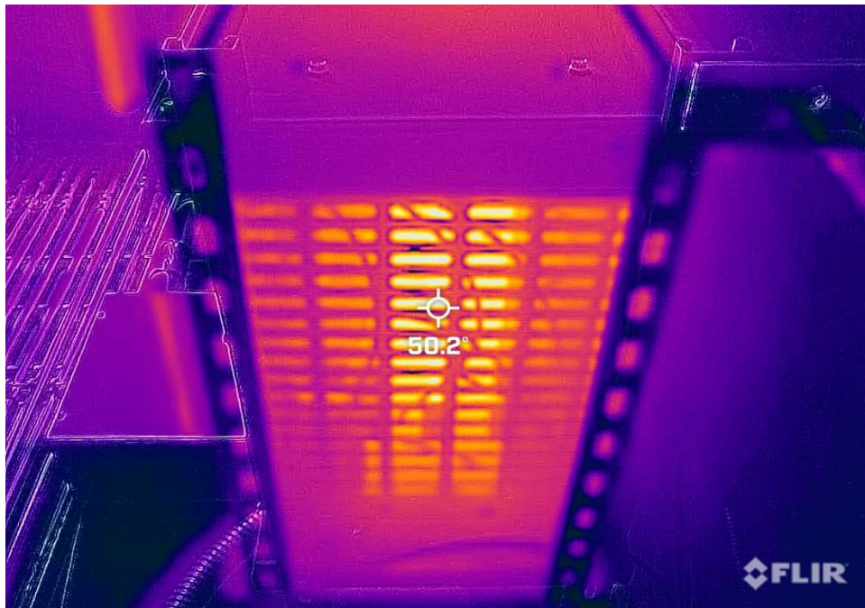
Item 55: T91 at 50.2 Degrees Celsius
