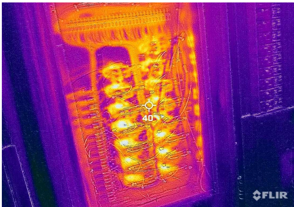
Item 54: Control Panel at 40.0 Degrees Celsius
