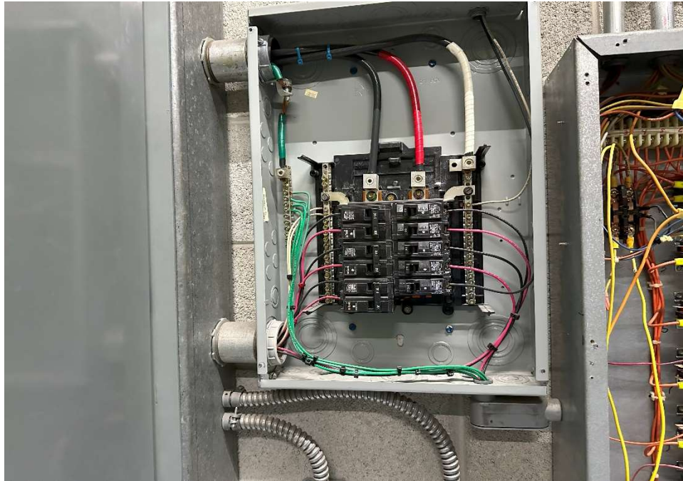
Panel NL2 Opened -
