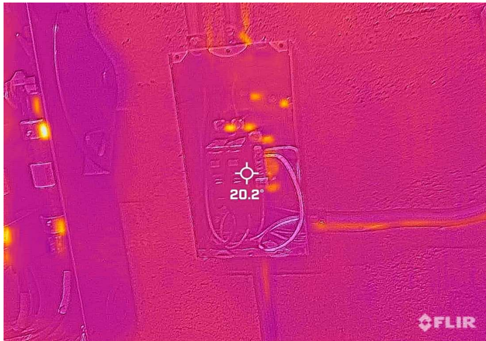
Item 29: Panel ELI at 30.0 Degrees Celsius (delta 0.2C)
