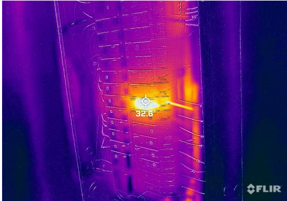
Item 37: Panel A at 32.6 Degrees Celsius (delta 7.6C)
