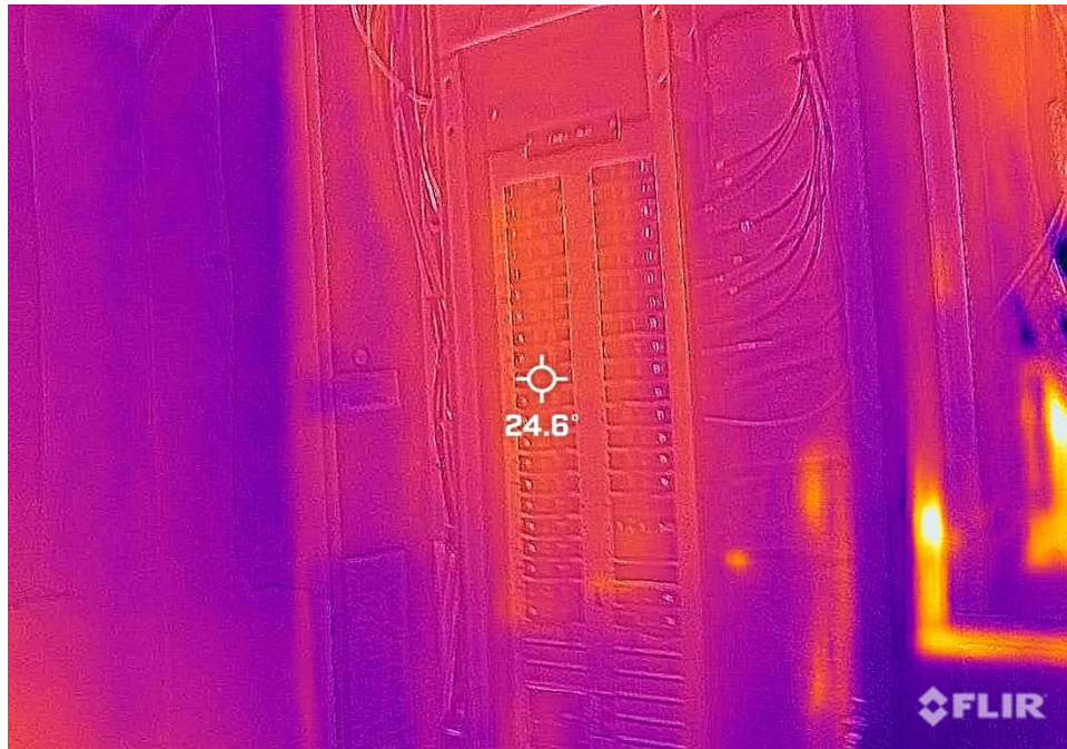
Item 57: Panel 1NL10 at 24.6 Degrees Celsius (delta 1.6C)
