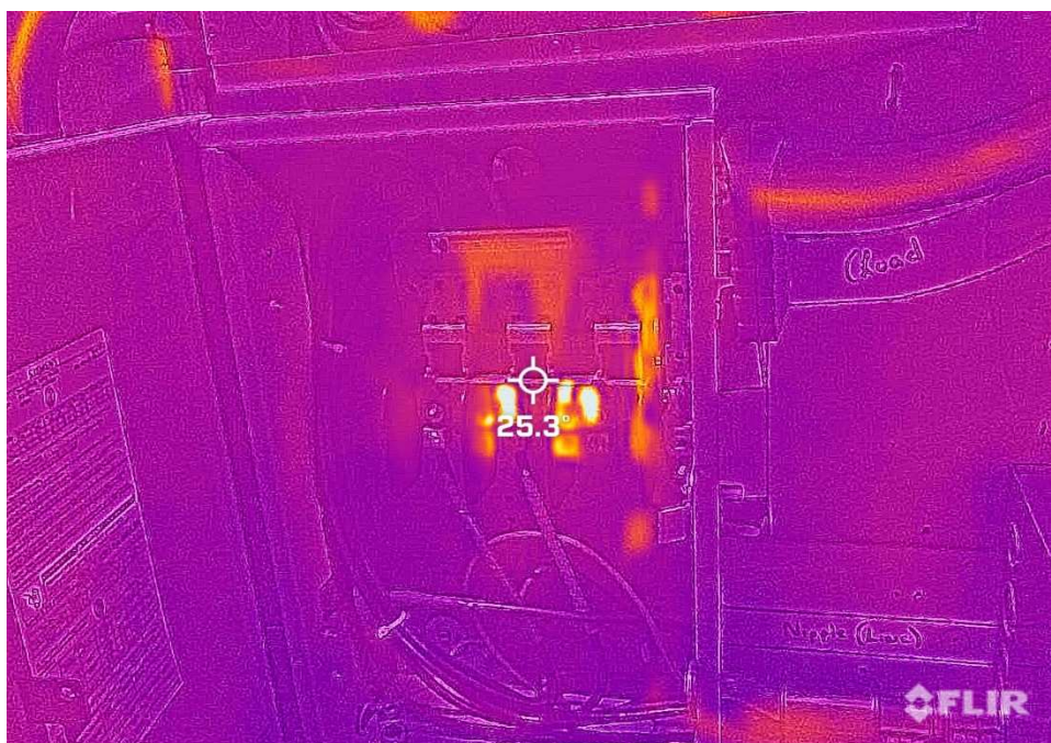
Item 77: Disconnect at 25.3 Degrees Celsius (delta 2.3C)
