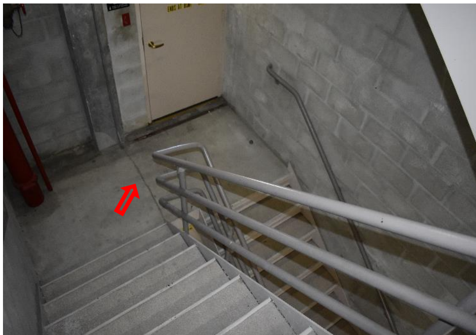
Typical cracks at the stair landing
