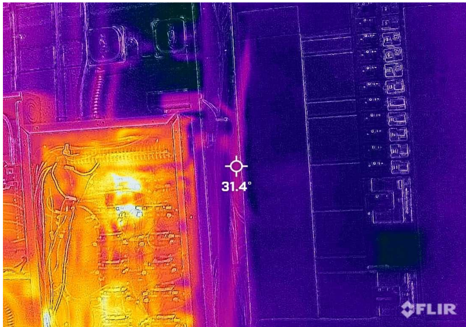
Item 8: Panel NH1 at 31.4 Degrees Celsius (delta 6.4C)
