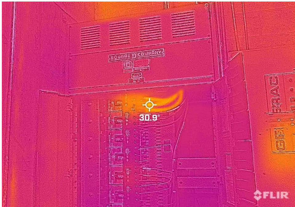
Item 21: Panel EDP at 30.9 Degrees Celsius (delta 5.9C)
