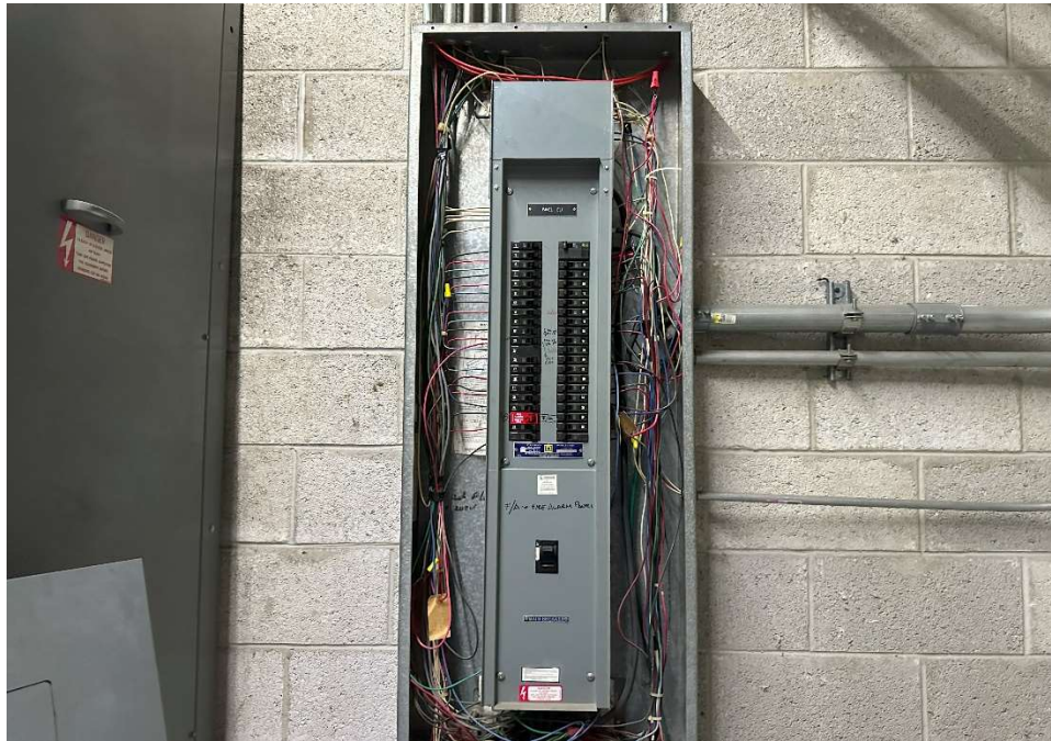
Main 5 of 5 Opened – 150 Amps – Emergency Main Panel EL1
