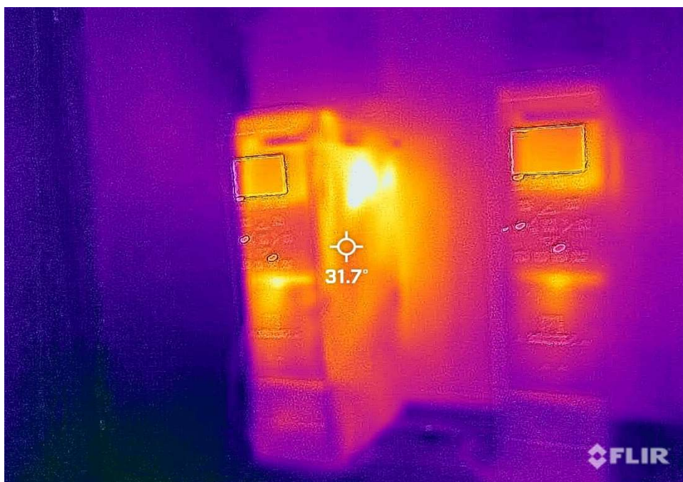
Item 17: VFD's at 31.7 Degrees Celsius (delta 6.7C)
