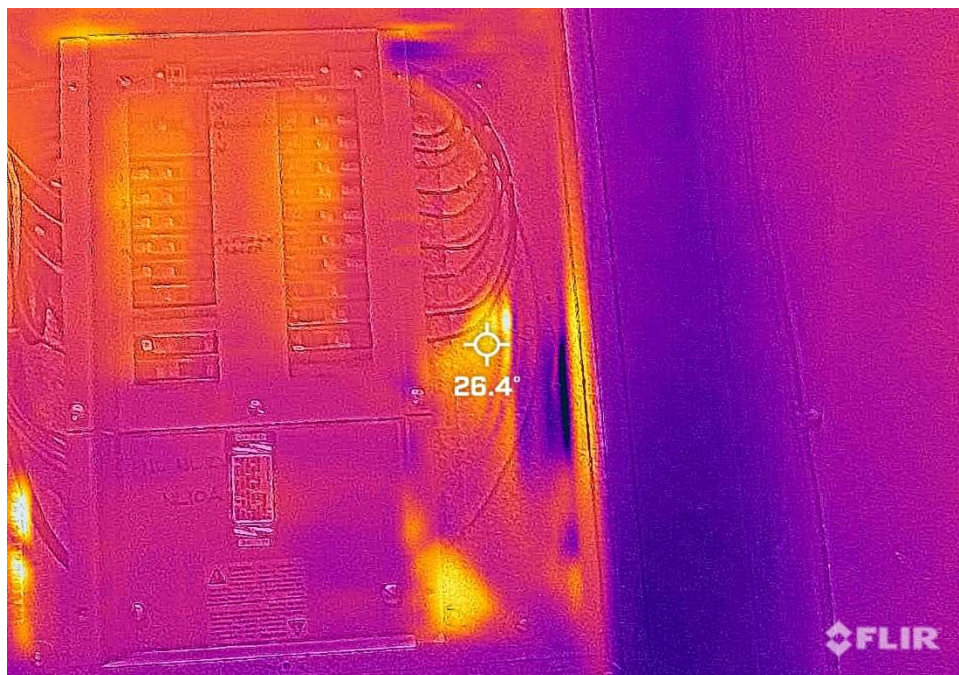
Item 58: Panel NL10A at 26.4 Degrees Celsius (delta 2.4C)
