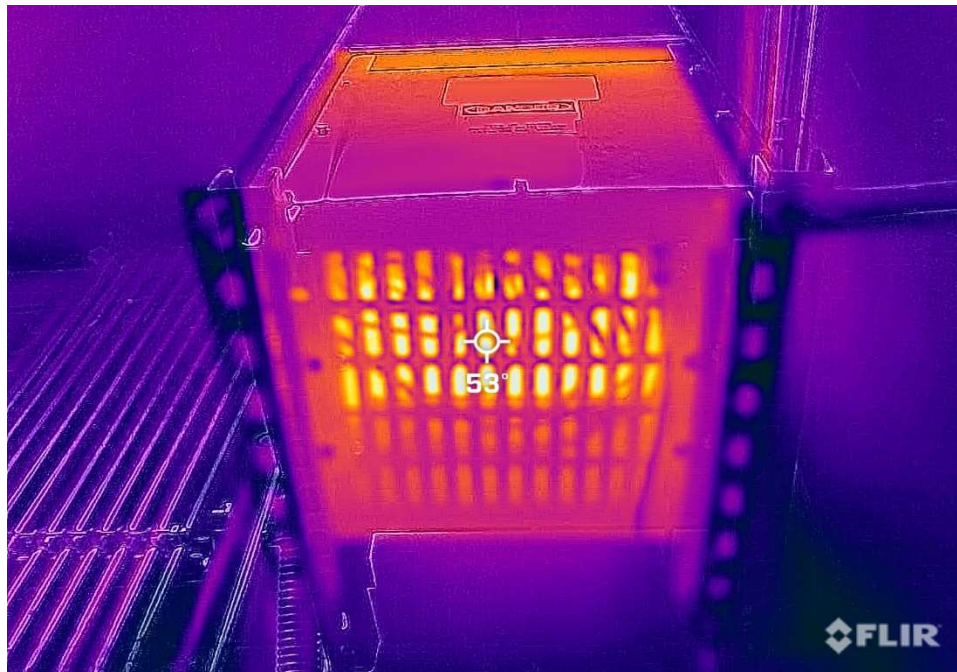
Item 63: T102 at 27.3 Degrees Celsius (delta 4.3C)
