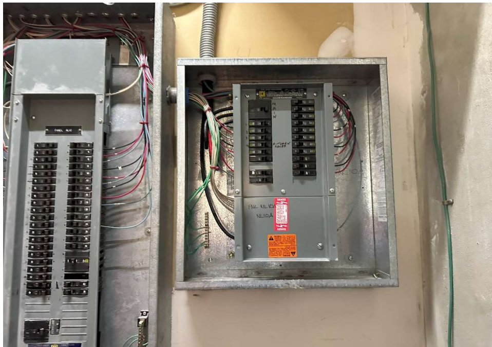
Panels NL10 and NL10A Opened -
