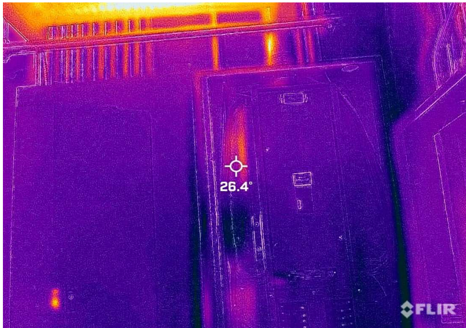
Item 66: Panel NH11A at 26.4 Degrees Celsius (delta 2.4C)
