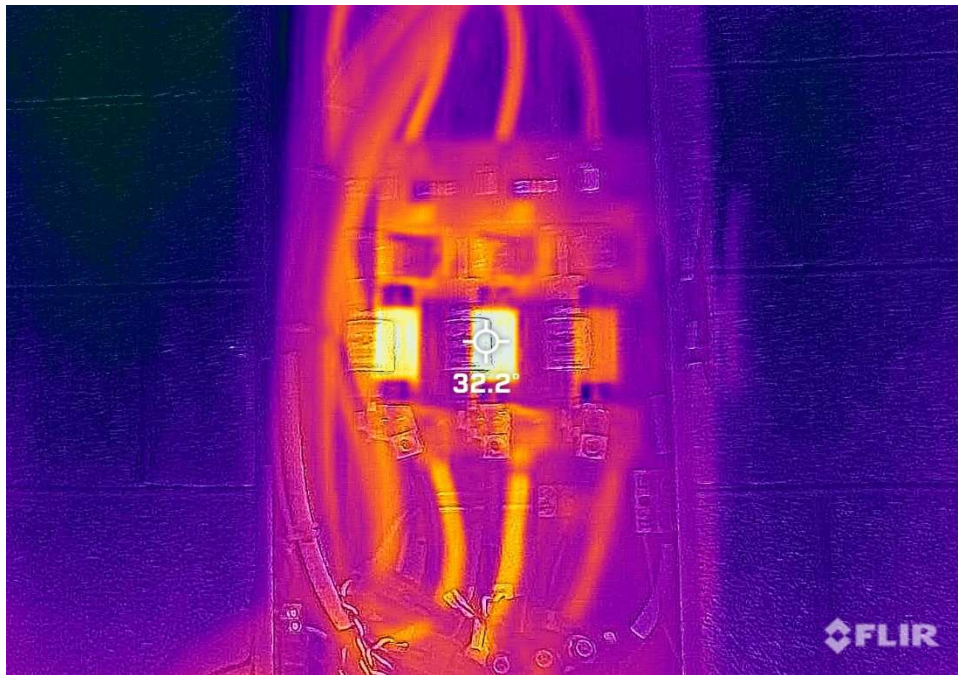
Item 14: Transformer Disconnect at 32.2 Degrees Celsius (delta 7.2C)
