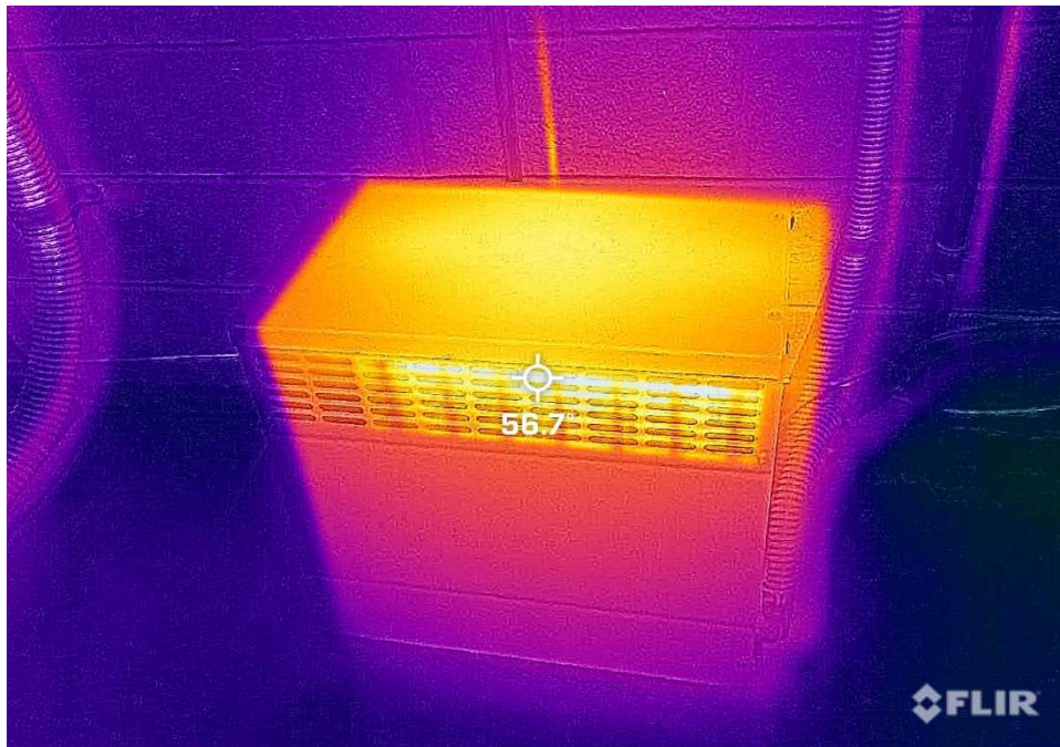
Item 15: T3 at 56.7 Degrees Celsius
