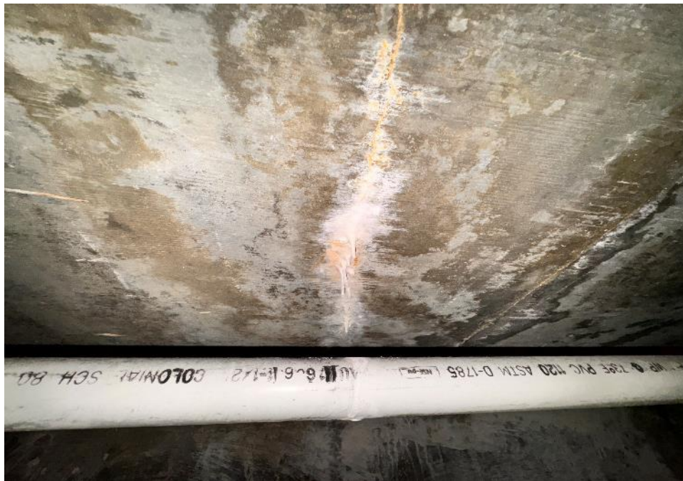
Typical cracks with efflorescence/moisture at the garage 2 nd level
