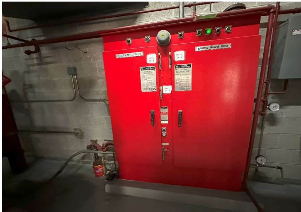
Fire Pump Control Cabinet -
