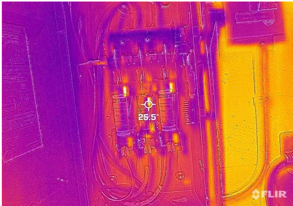
Item 22: Elev Disconnect 1 at 25.5 Degrees Celsius (delta 3.5C)
