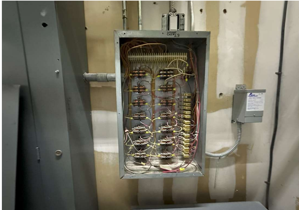
Relay Control Panel Opened -
