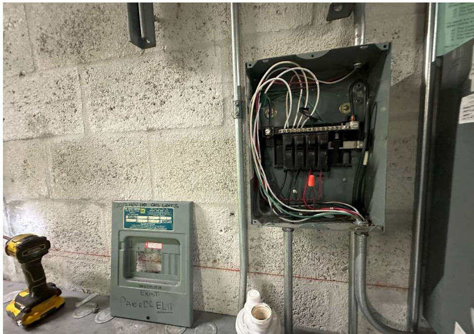
Panel EL II (Elev Cab Lights) Opened -
