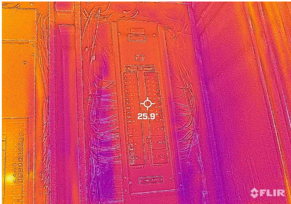
Item 74: Panel N12R at 25.9 Degrees Celsius (delta 3.9C)
