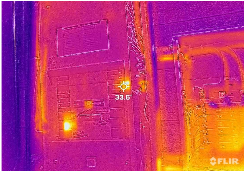
Item 11: Panel NL1 at 33.6 Degrees Celsius (delta 8.6C)
