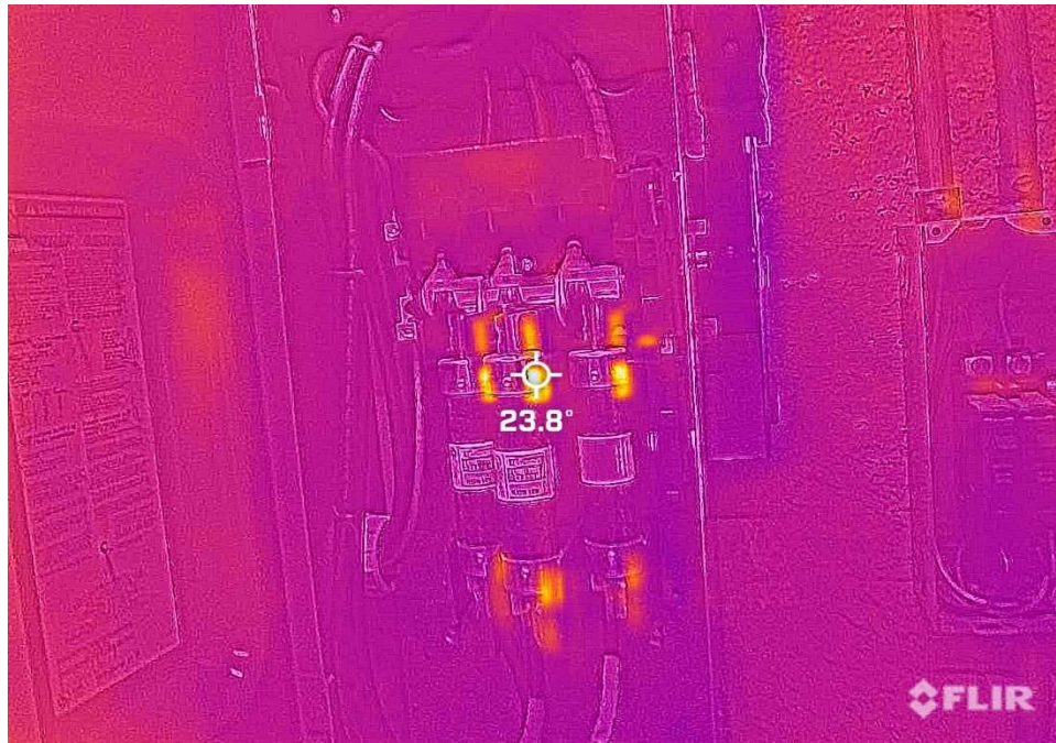
Item 28: Elevator 4 Disconnect at 23.8 Degrees Celsius (delta 1.8C)
