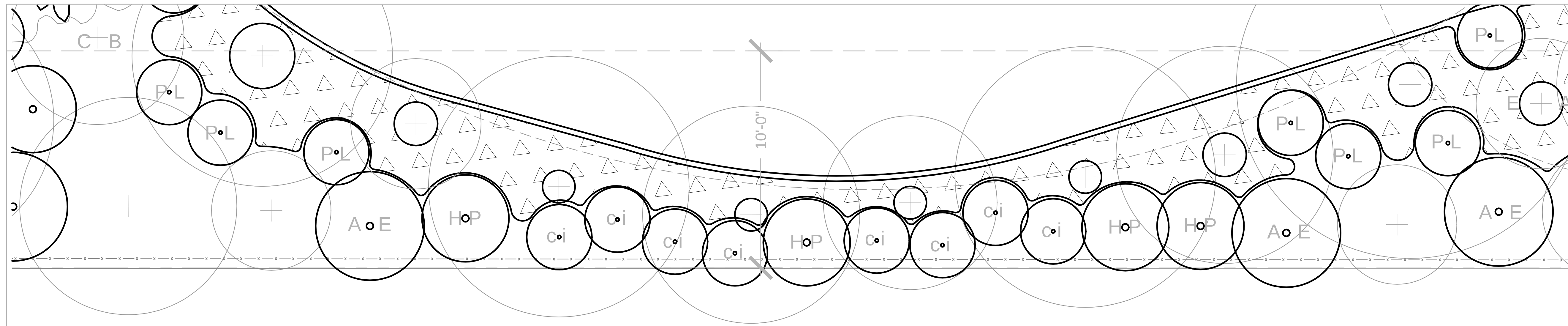
VILLA SERENA: SHRUBS AND GROUND COVERS PLANTING PLAN SCALE: 1/2"=1'
