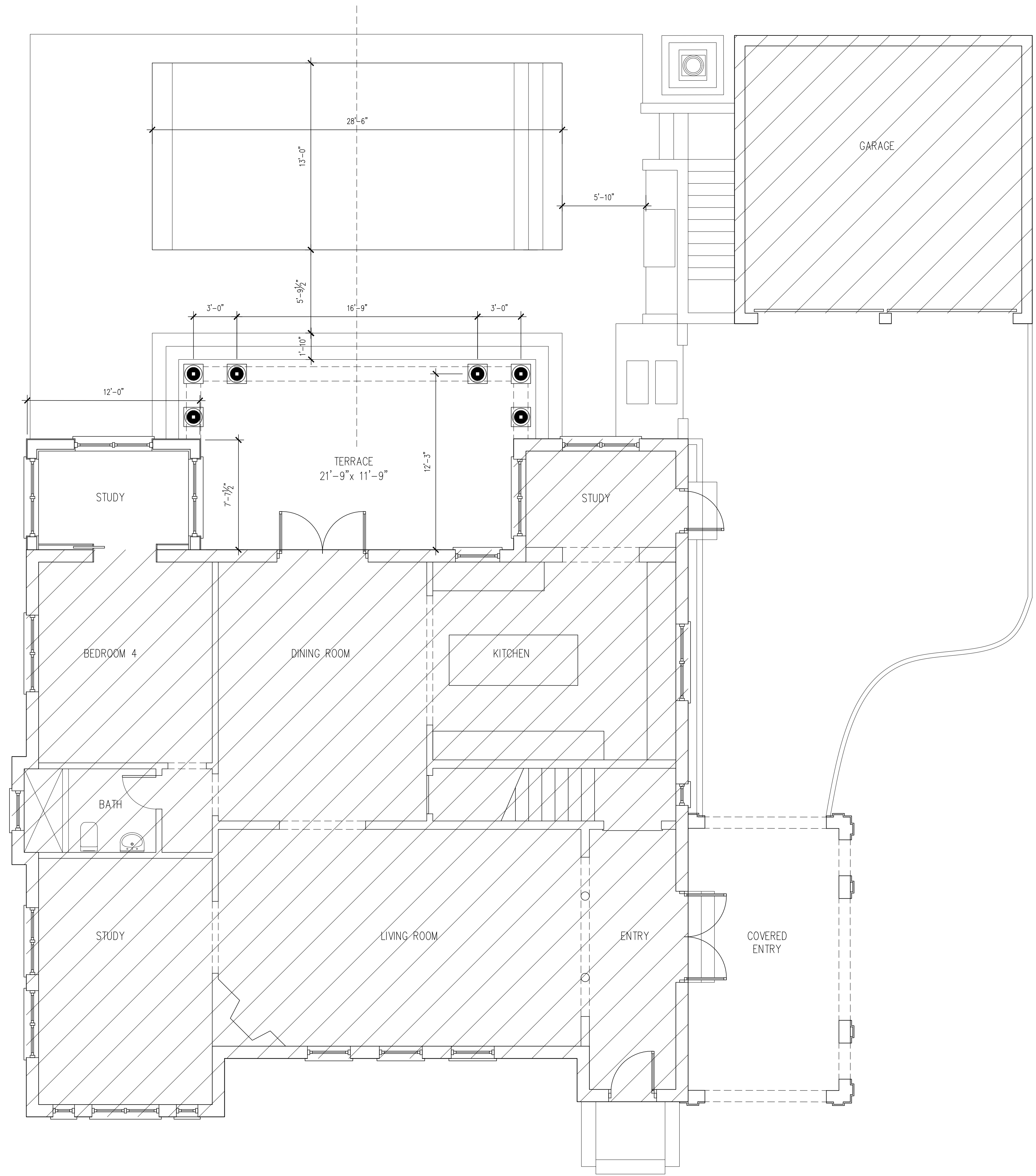
PROPOSED GROUND FLOOR PLAN 1/4"
